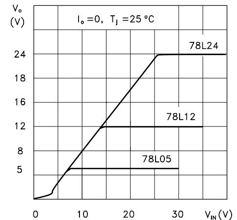
Figure 6 : Output Characteristics
